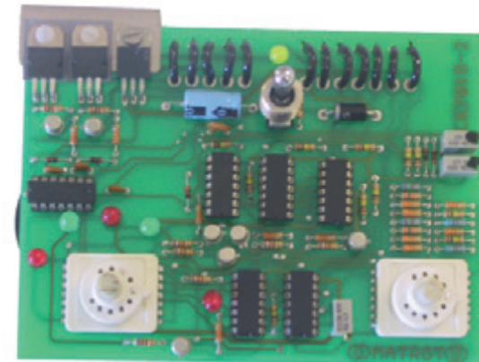
Circuit imprimé Direction Direction printed circuit Ref 007 015 100
